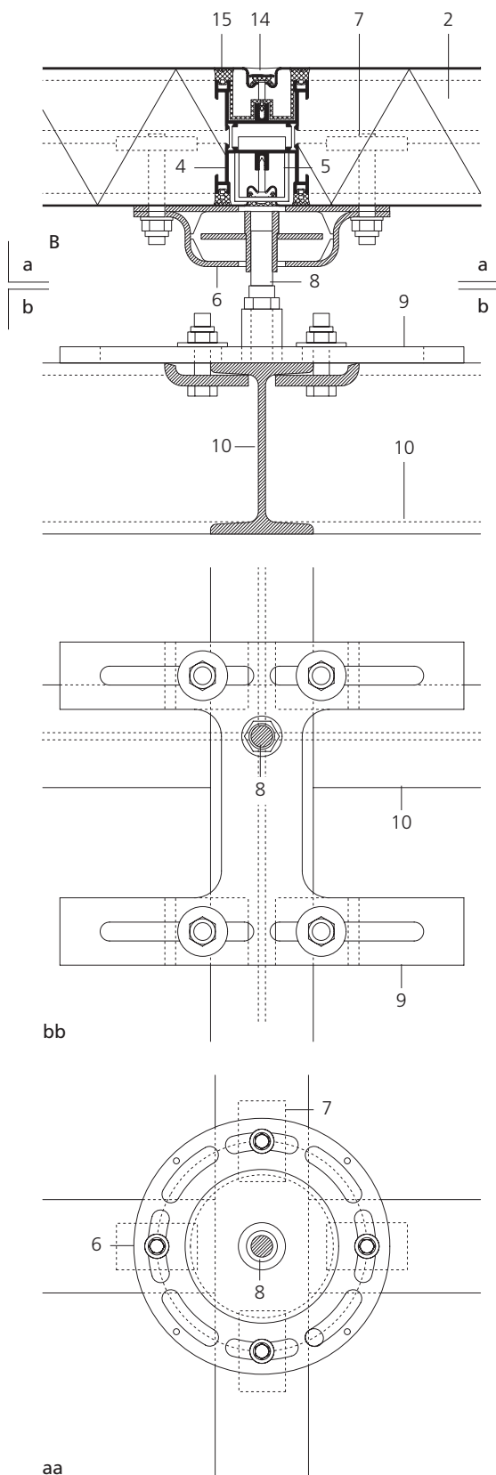
Details of façade panels scale 1:5
