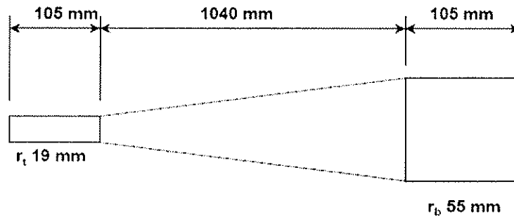
Fig 5 The tubular blank for the hydroformed concept
